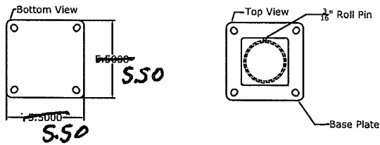
1.875 x 1.875 Structural Post
