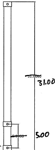
1.875 x 1.875 Side Mount Structural Post
