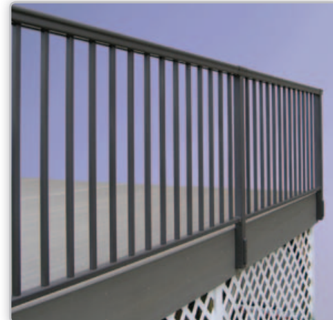
Over The Post (OTP) Side/Fascia Mount
